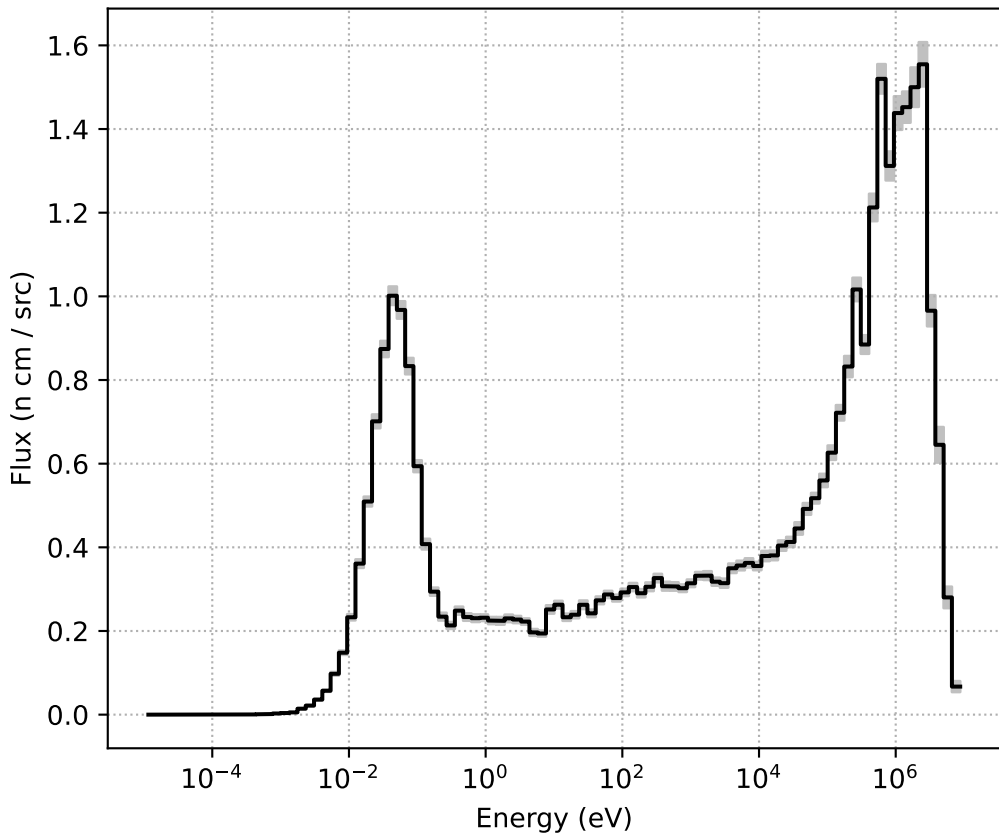
Neutron Energy Flux
